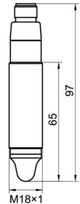
M18 x 1 ISO 261 / ISO 965 (BCID: M11)
